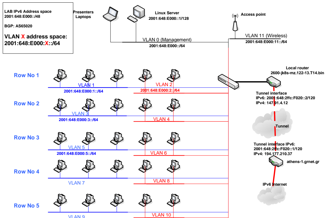
Figure 1: Lab topology
